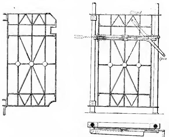
Figs. 3797-3800. Plan and Elevations. GOLD'S PLATFORM GATE.
